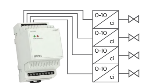
control via Digital/analog converter DAC3-04M
